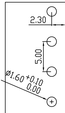
PCB LAYOUT
