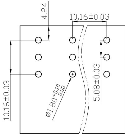
PCB LAYOUT
