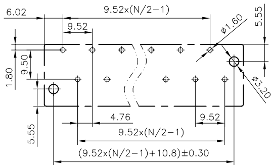
PCB LAYOUT
